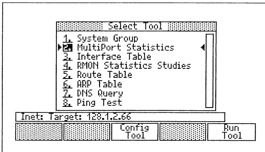
Figure 9-11. Toolkit Menu
